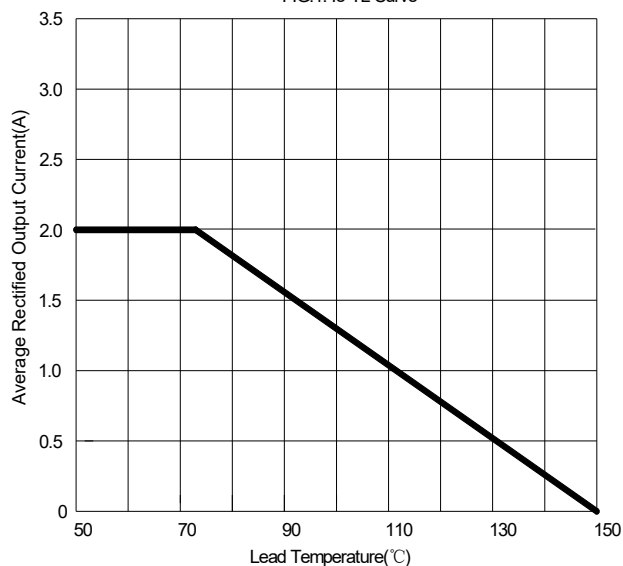
FIG.1: Io-TL Curve
